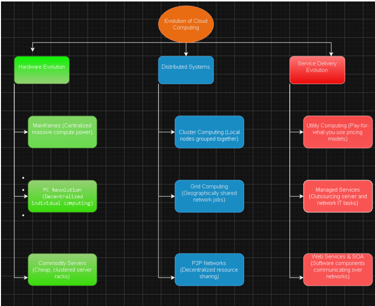
Concept Map 2: Evolution of Cloud Computing
